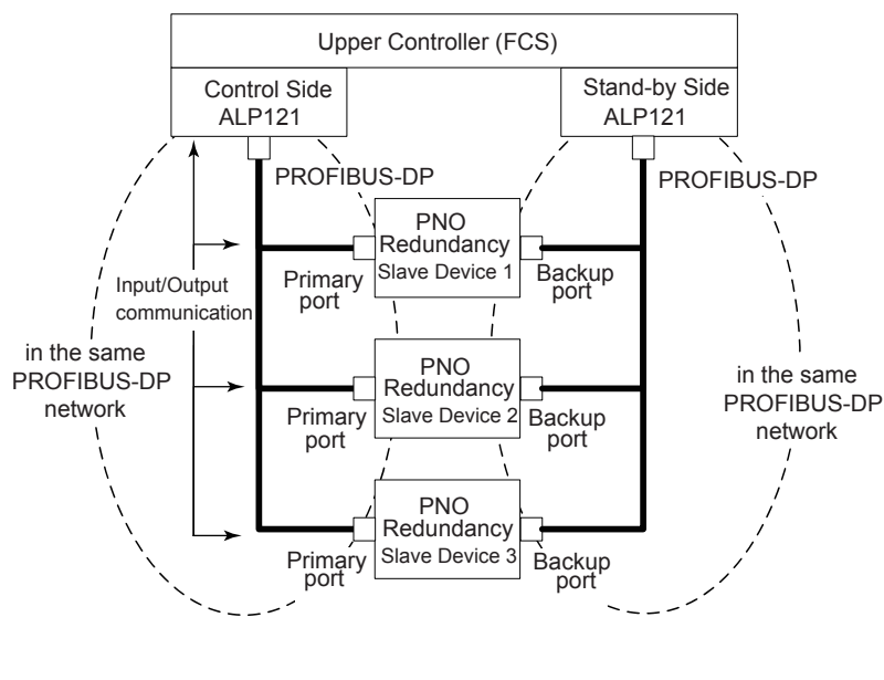
Figure Dual-redundant Configuration of the PROFIBUS-DP Communication Module
